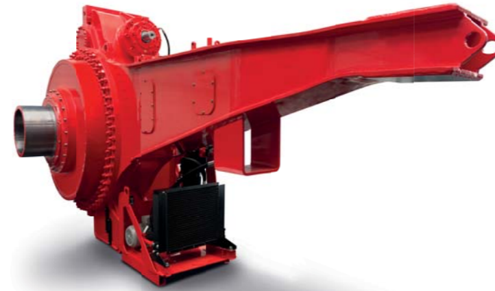
Bevel-helical-planetary bucket wheel drive
