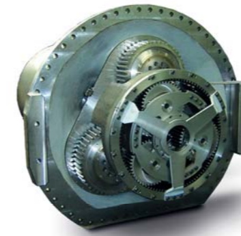
Planetary haul truck axle gearbox
