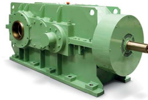
Belt conveyor bevel-helical gear unit
